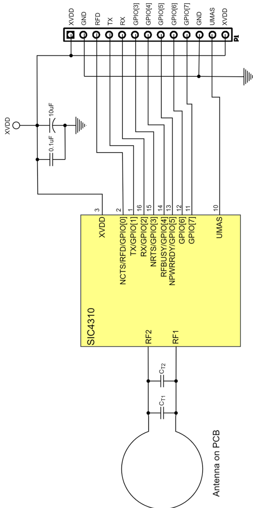
Figure 2: Simplified schematic diagram of SIC4310-HV
