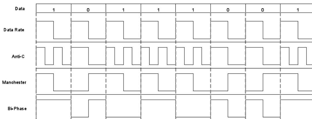
Figure 6-3: Coding Techniques of SIC278 Transponder
