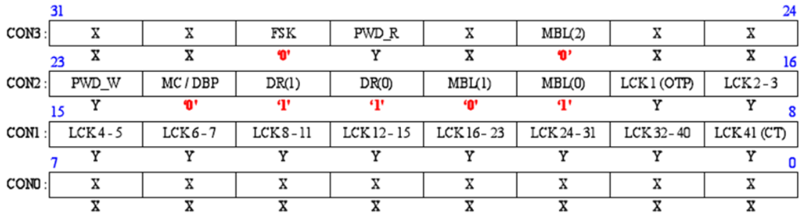
Figure 8-7: Configuration for 64-bit ID TTF with Manchester coding
