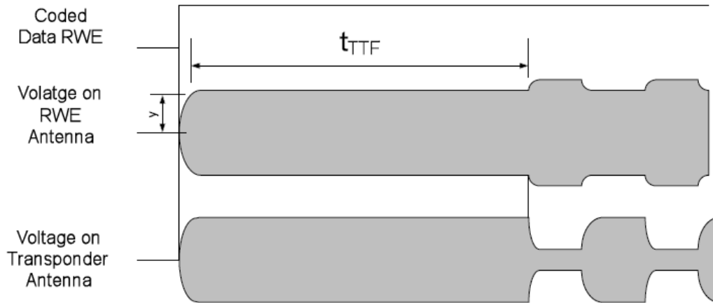
Figure 6-8: SIC278 Waiting Time before transmitting data in TTF Mode
