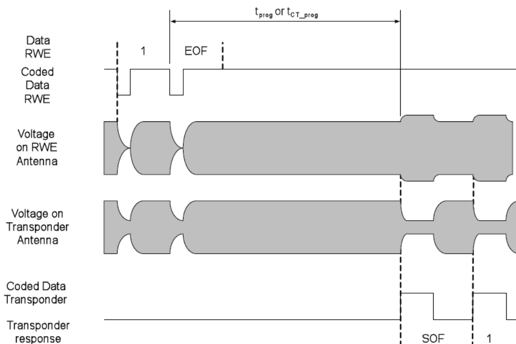
Figure 6-7: SIC278 Transponder Programming Time
