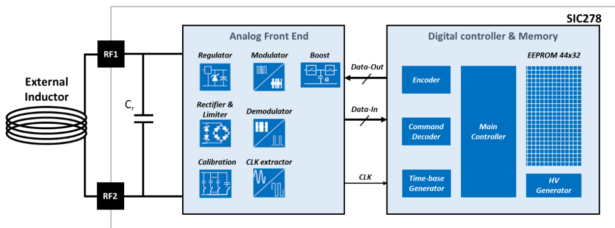
Figure 1-1: SIC278 Functional block diagram
