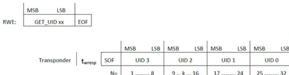
Figure 7-1: GET_UID Bit Stream
