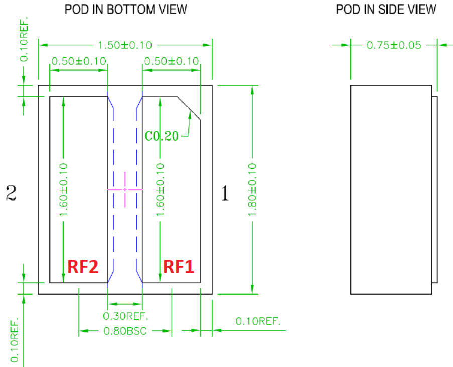
Figure 10-1: WDFN 1.5x1.8 mm Package Drawing
