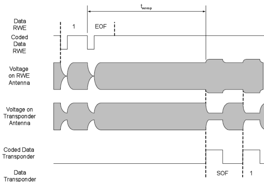
Figure 6-6: SIC278 Waiting Time before transmitting a response after receiving an EOF
