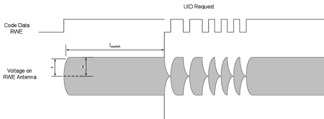
Figure 6-9: SIC278 Transponder Mode Switching Time
