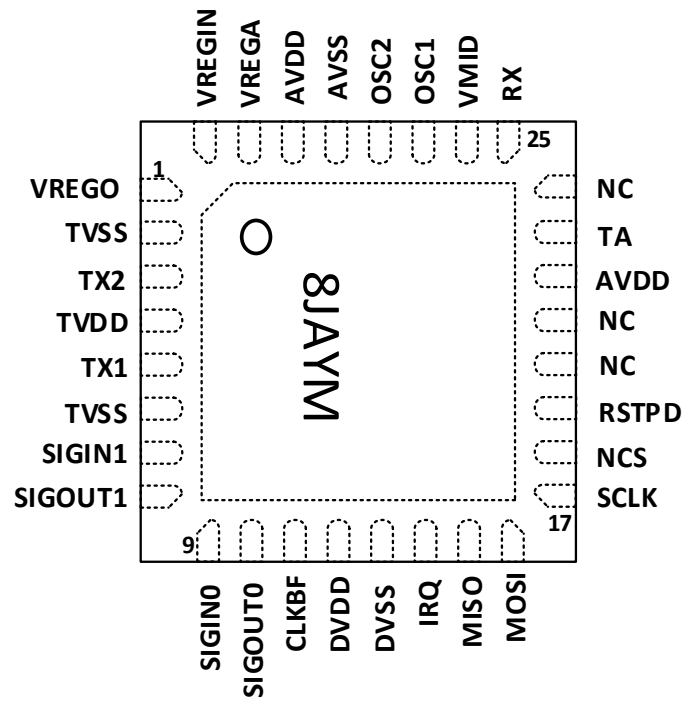
Figure 4 Pin arrangement (top view)
