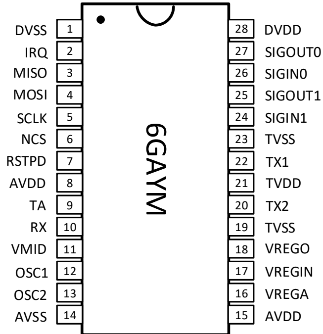
Figure 5 TSSOP Pin arrangement (top view)
