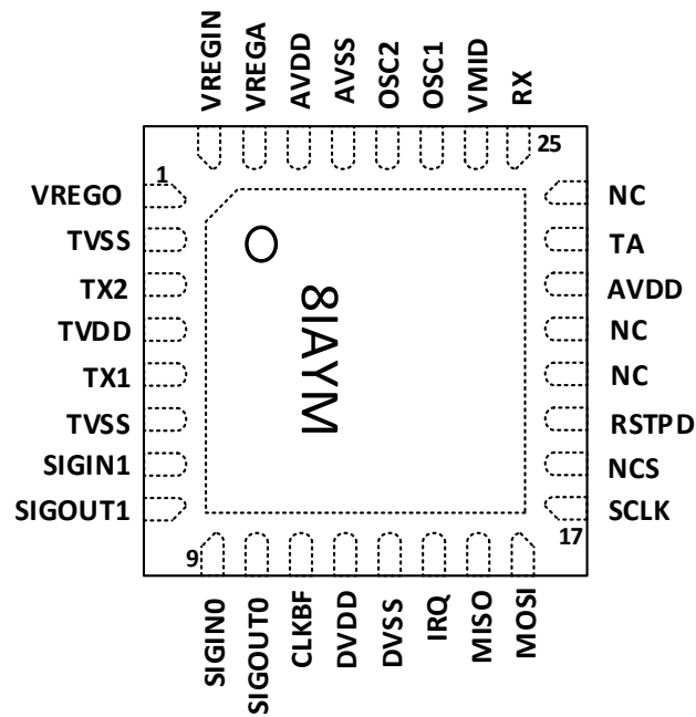
Figure 4 Pin arrangement (top view)
